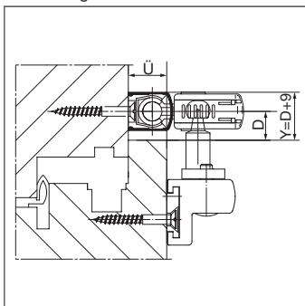
GEZE OL 95 an Holzfenster Euronut
