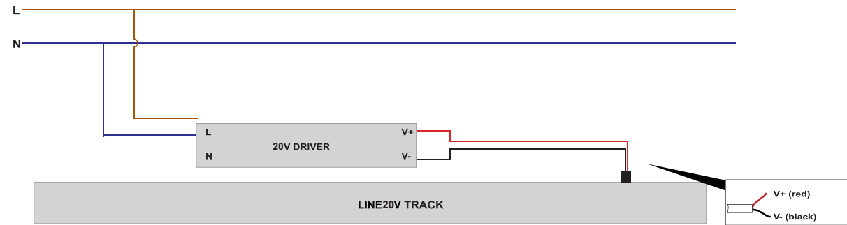
LINE20V-ON-OFF-Wiring Diagram
