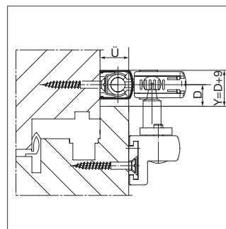
GEZE OL 90 N an Holzfenster Euronut
